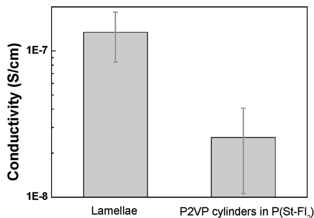
Figure 8. Effect of morphology on the conductivity of P(St-Fl 2 )- b -P2VP/P3-SWCNT (2 wt %). P(St-Fl)- b -P2VP-1 shows the lamellae structure, and P(St-Fl 2 )- b -P2VP-1 shows the P2VP cylinders in the P(St-Fl 2 ) matrix.
